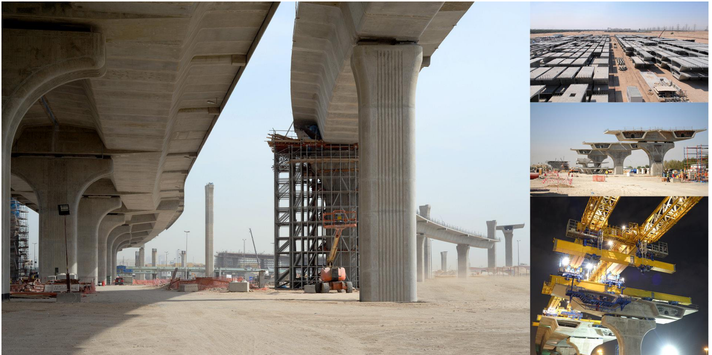
Continuous viaducts with segmental construction overall length 11 km, typical span: 45.00 m.
